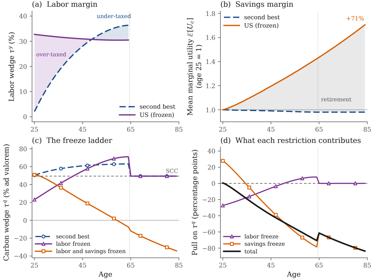
Figure 3: The two frozen schedules and what they do to the carbon wedge. The benchmark \tau^k = 0.18 throughout, and a pull is the difference between consecutive paths in (c). Blue is the unrestricted second best, purple the labor restriction, orange the savings restriction, black their total; the second best is dashed and anything frozen is solid. (a) The frozen labor schedule at its age- t anchor against the second-best wedge at the same age; shading takes the color of whichever curve is on top, purple where the frozen schedule overdistorts labor and blue where it underdistorts. (b) The savings margin as the accumulated distortion: mean marginal utility under each regime, indexed to one at age 25, with the grey band the gap between them. Levels of U_c are not comparable across allocations; (11) restricts the growth rate, which is what the panel plots. The shading is neutral because a frozen savings wedge constrains a ratio across dates, so its multiplier changes sign (Lemma 5.3) and this gap's sign does not map into the sign of the pull. Both retirement segments are analytical: the second best holds \mathbb{E}[U_c] constant once risk resolves, and the frozen path compounds at 1/(1 - \bar{\tau}^s) . (c) The carbon wedge with nothing frozen, with the labor schedule frozen, and with both margins frozen; the retirement segments of the first two paths are analytical (Appendix C.12). (d) The two pulls, which sum to the total at every age.
