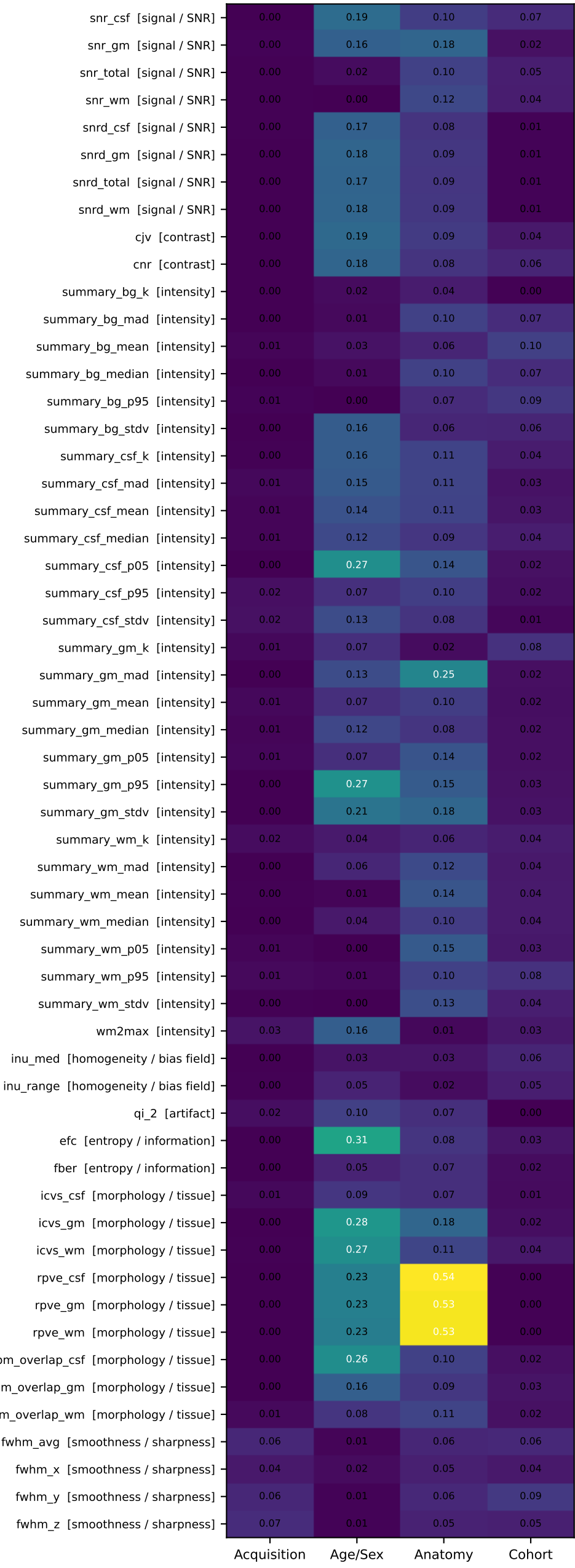
Incremental R 2 by predictor family (OLS; not causal)
