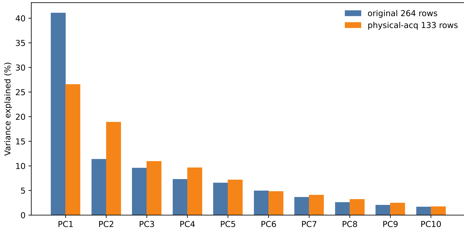
T1w IQM PCA variance: original vs physical-acquisition
