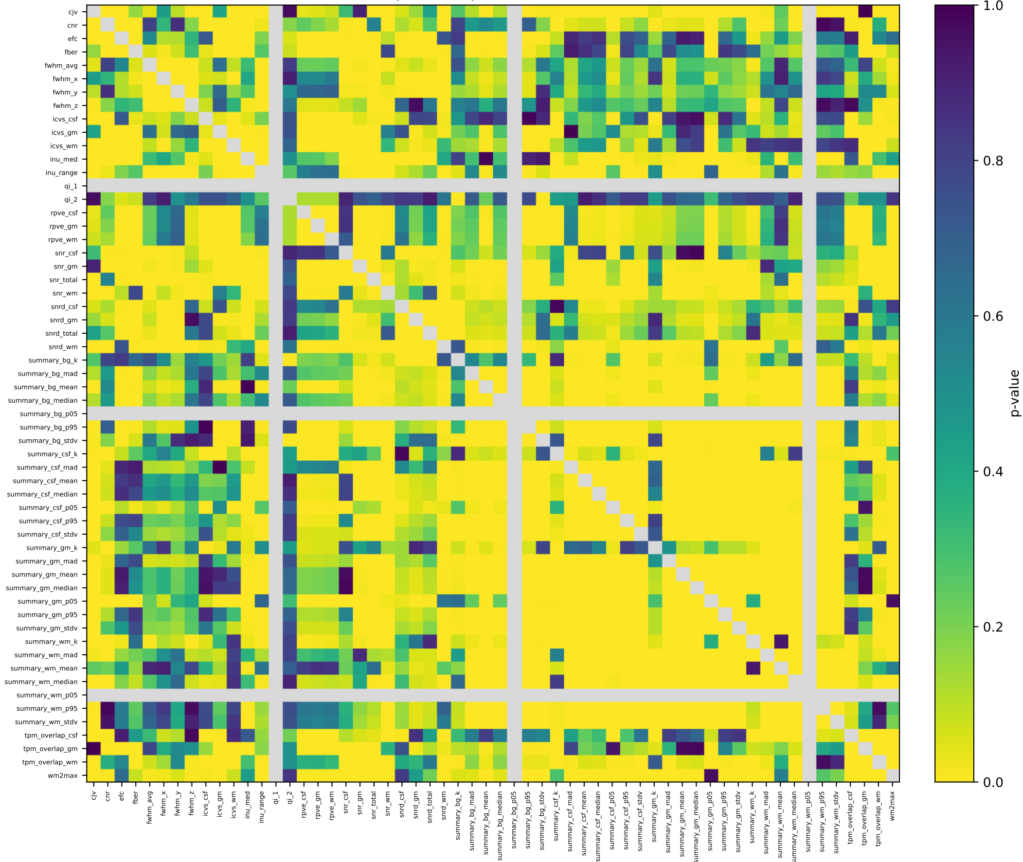
Spearman p-values — WMn
