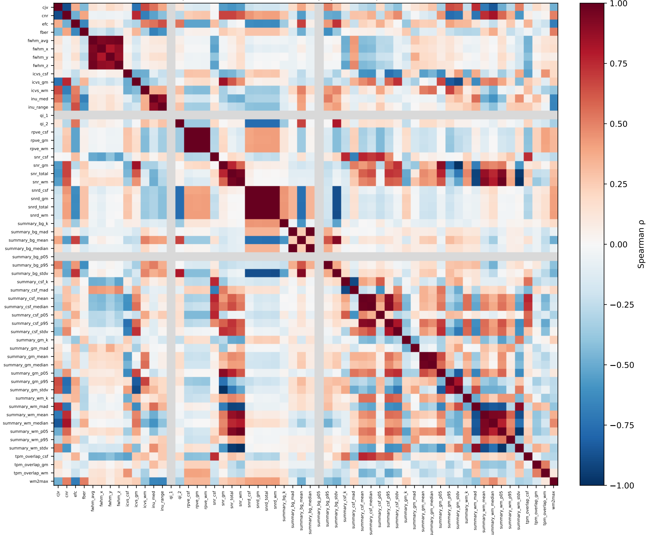
Spearman IQM correlation — physical-acquisition T1w
