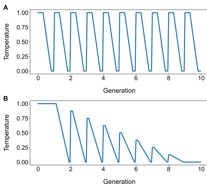
Fig. 3.2: A: Annealing during a HYBRID run with global annealing turned off, i.e. using -maxiter 10 -temp 5 -anneal_begin 0.3 -anneal_end 0.8 . B: With global annealing turned on, i.e. using -maxiter 10 -temp 5 -anneal_begin 0.1 -anneal_end 0.9 -anneal_global_begin 0.1 -anneal_global_end 0.9 .
