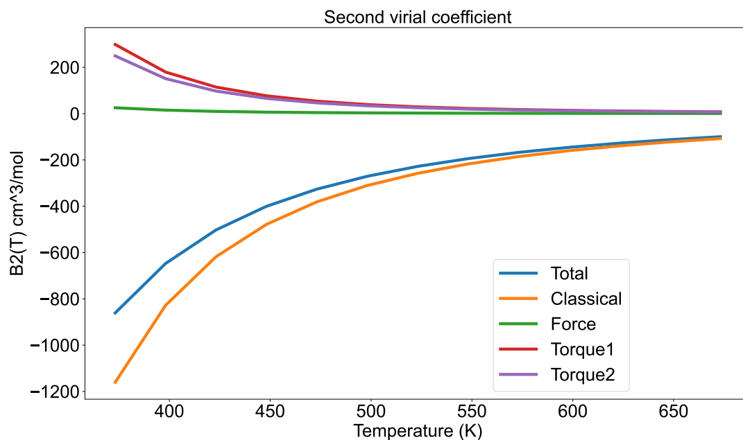
Fig. 2.8: Sample second virial coefficient and components for water using the TIP4P model.
