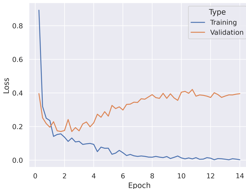
Figura 6: Training e Validation Loss - Fine-tuning Completo
