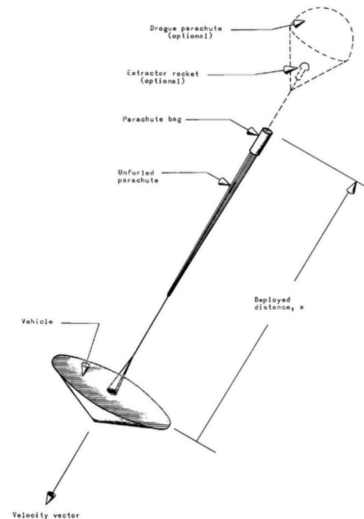
Figure 1.- Sketch of deployment configuration.
