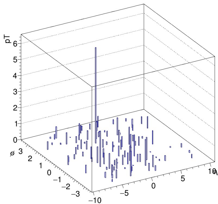
pT Distribution
