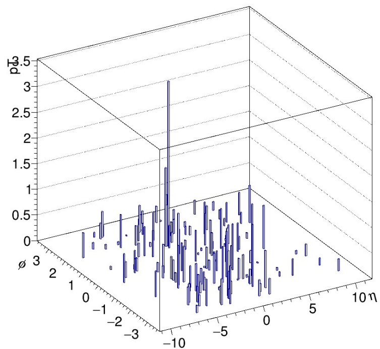
pT Distribution
