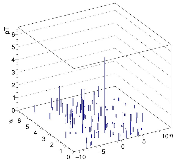
pT Distribution
