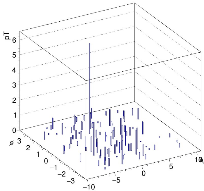
pT Distribution
