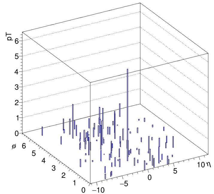
pT Distribution
