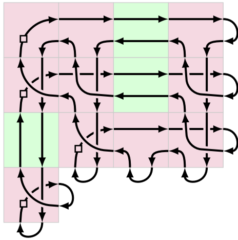
L_G^{\text{plab}}
