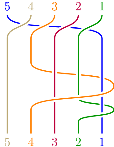
(e) \beta = \beta(\mathbf{a}(C))
