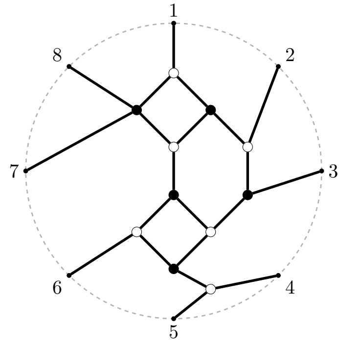
(a) Plabic graph G
