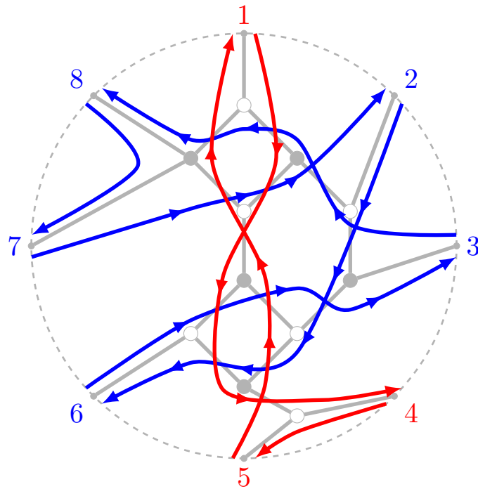
(b) Strands in G
