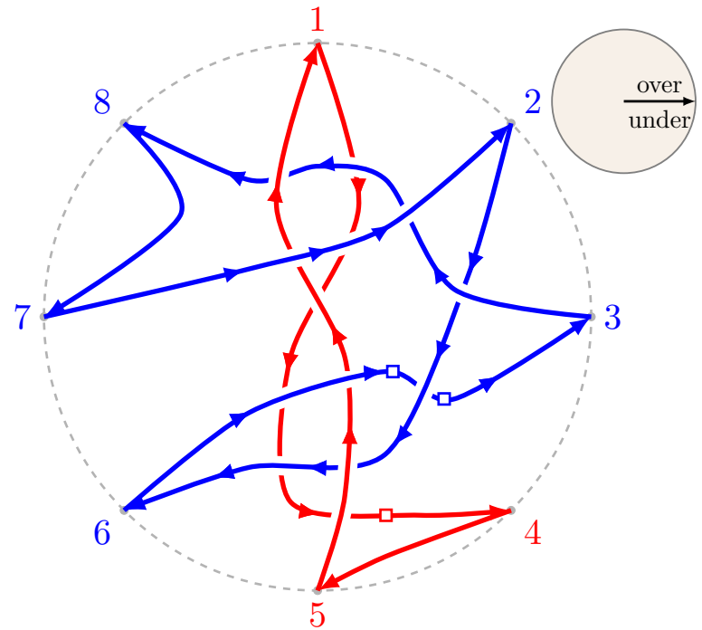
(c) Link L_G^{\text{plab}}
