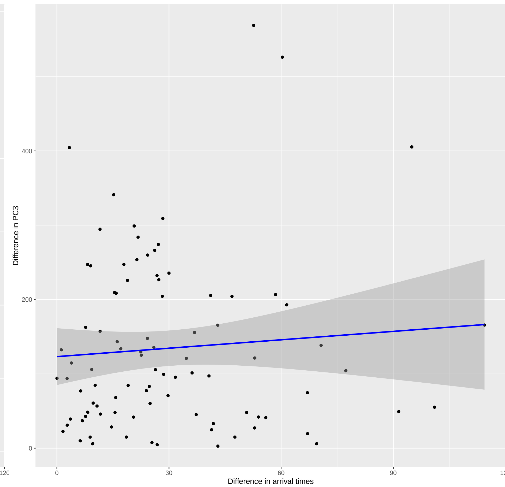
Model 2: hierarchical structure; \rho = 0.055
