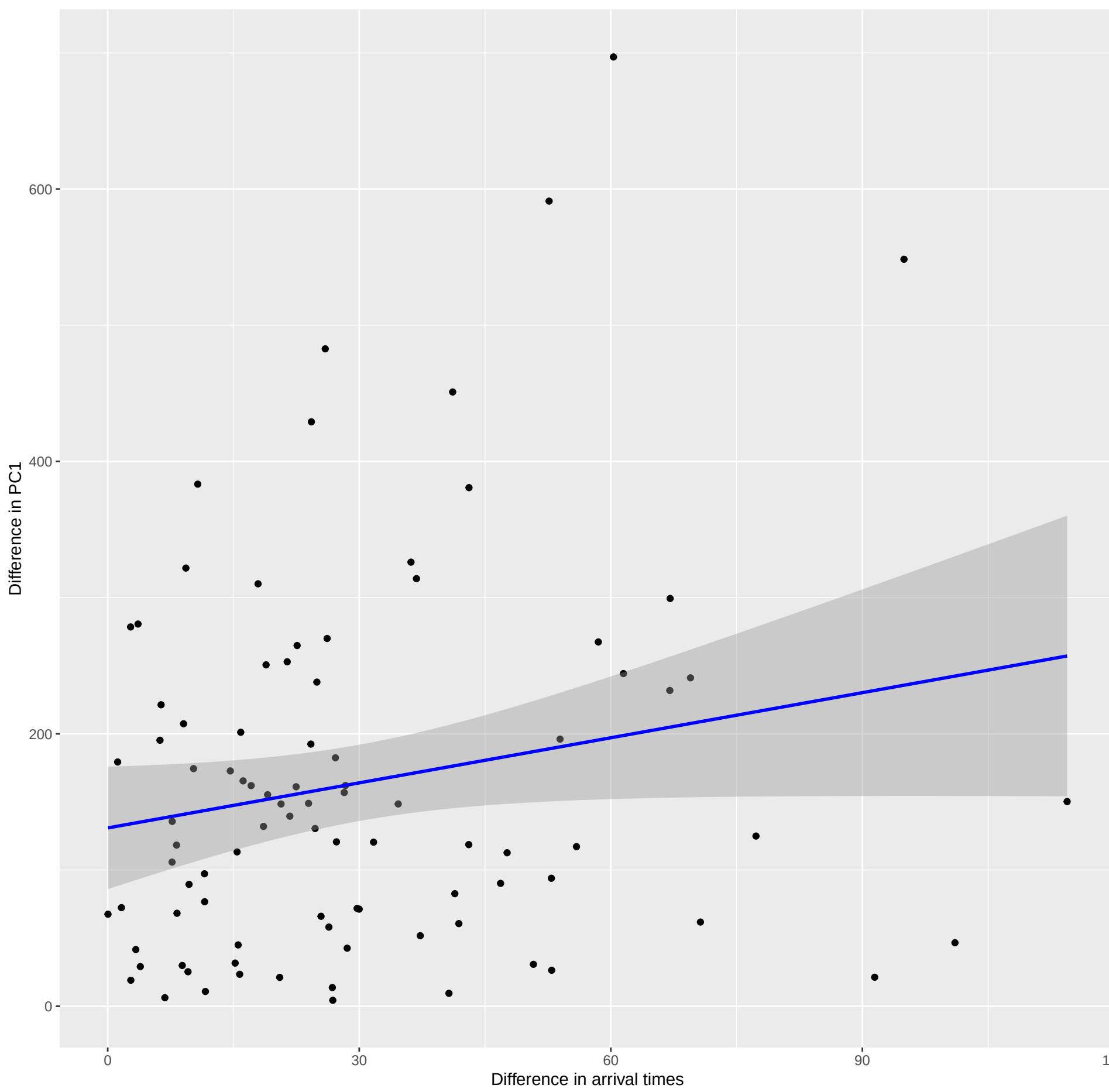
Model 2: hierarchical structure; \rho = 0.129
