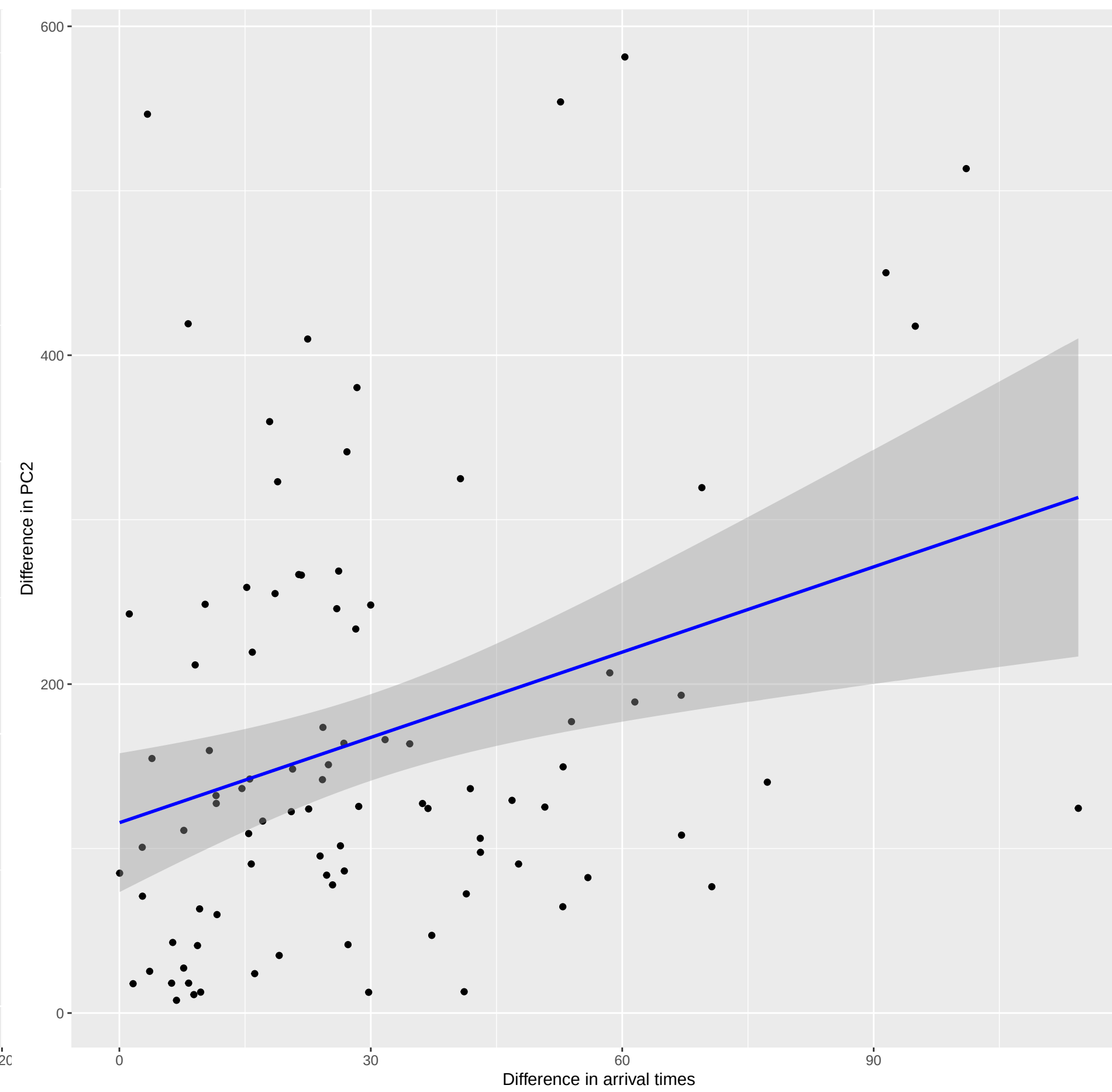
Model 2: hierarchical structure; \rho = 0.276
