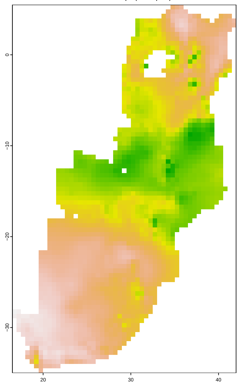
P of coldest qtr (mm qtr -1 )
