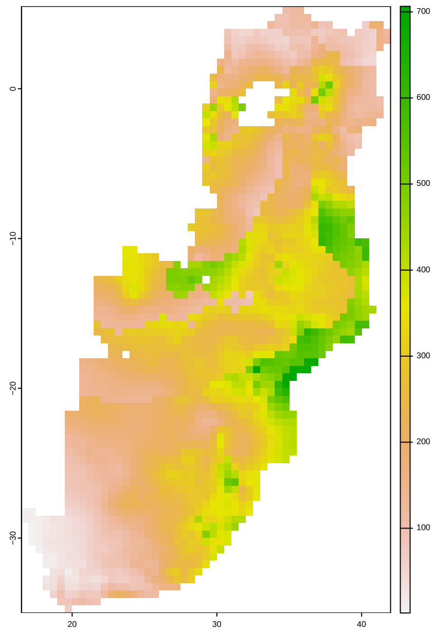
LAI (gC m -2 )
