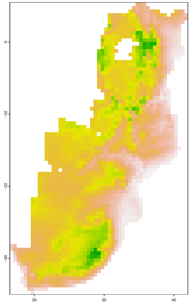
altitude over the sea level (m)
