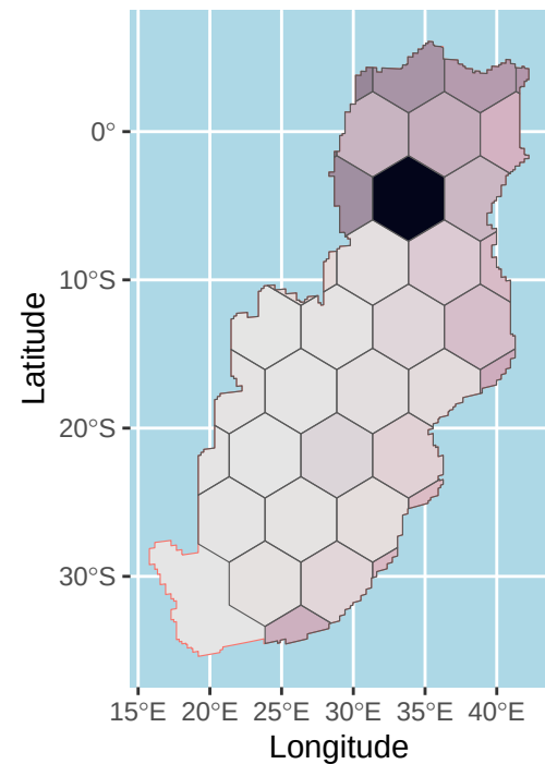
t = 2200 BP
