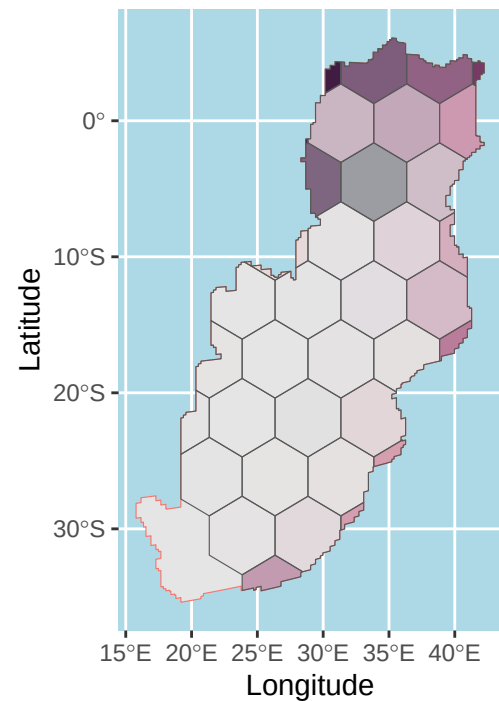
t = 1400 BP
