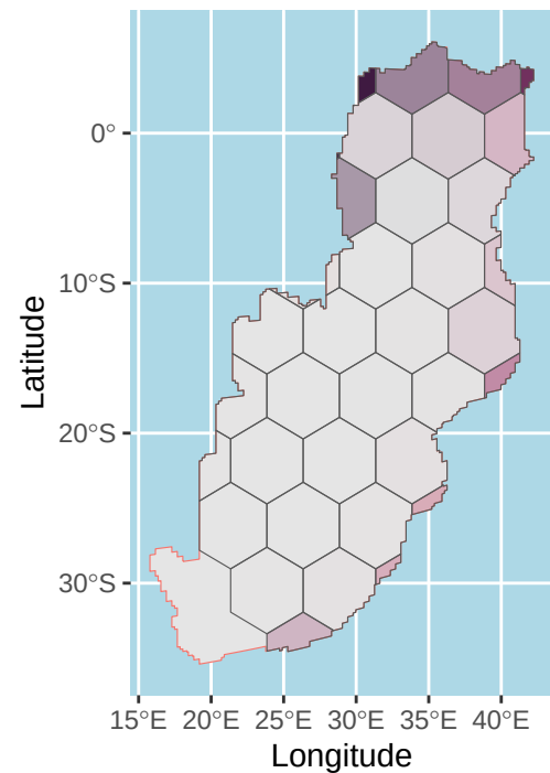
t = 1600 BP
