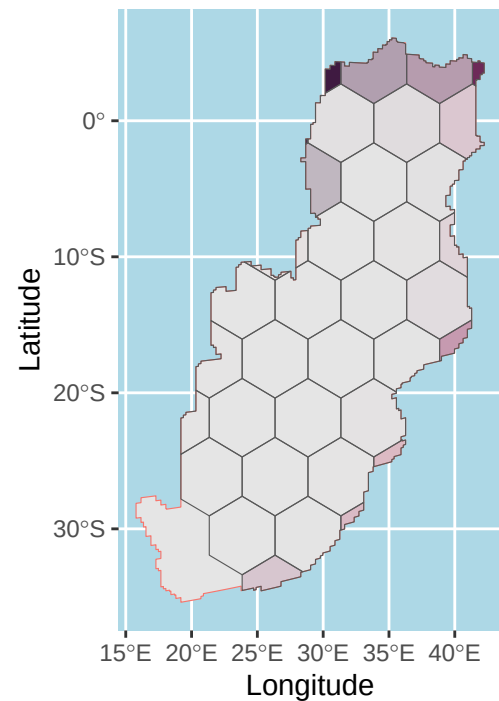
t = 1800 BP
