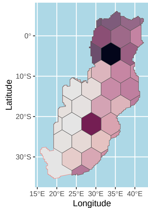
t = 2000 BP
