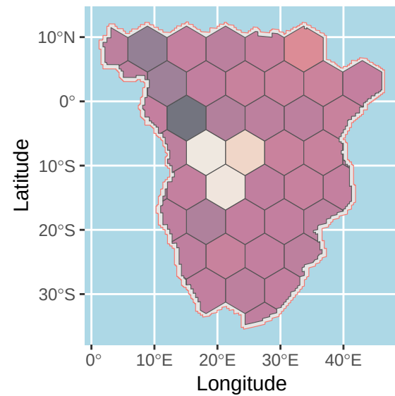
t = 3000 BP
