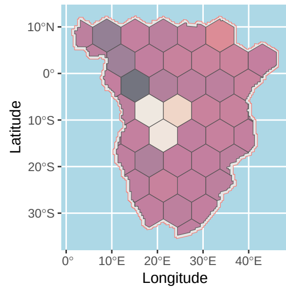
t = 2800 BP
