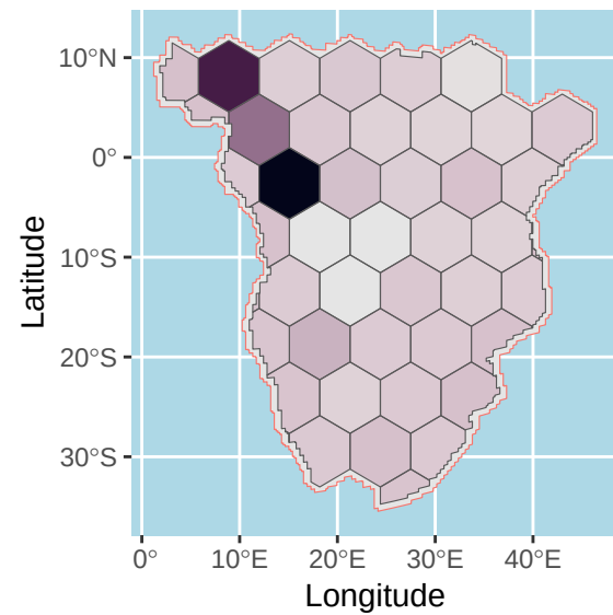
t = 2400 BP
