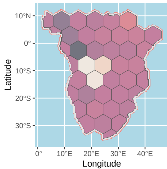
t = 3200 BP
