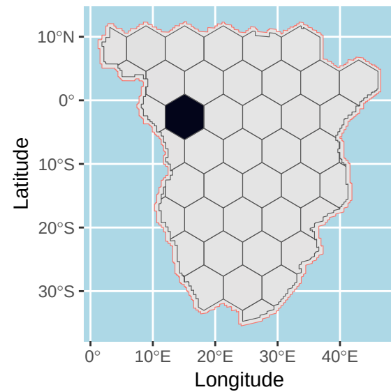
t = 2600 BP
