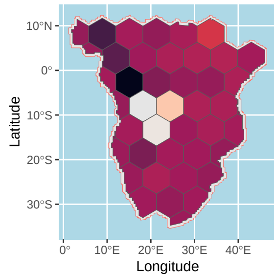
t = 1800 BP
