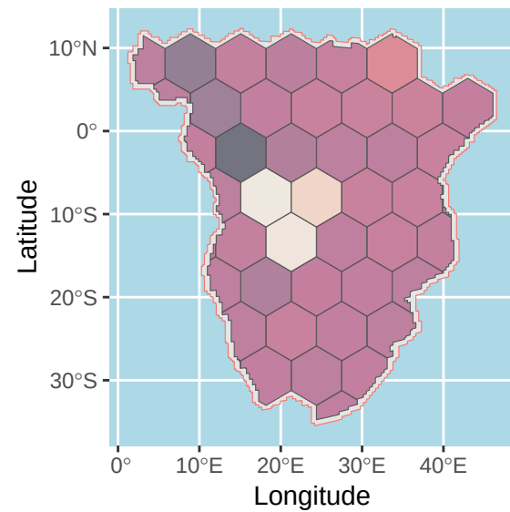
t = 1400 BP
