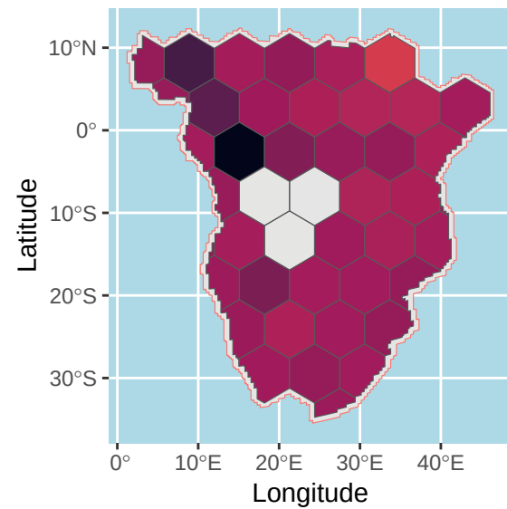
t = 2000 BP
