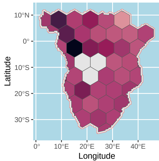
t = 2200 BP
