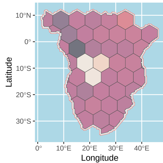
t = 1600 BP
