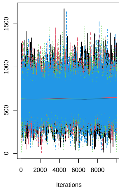
\nabla[24]
