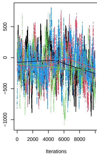
beta2
