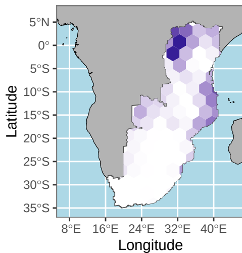
t = 2000 BP
