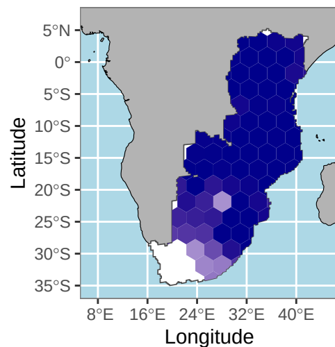
t = 1400 BP
