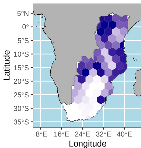
t = 1550 BP
