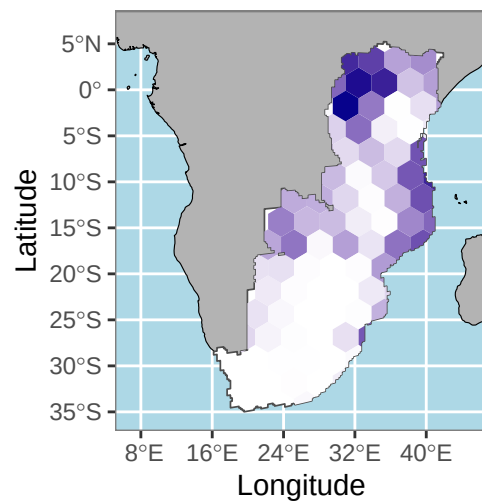
t = 1850 BP
