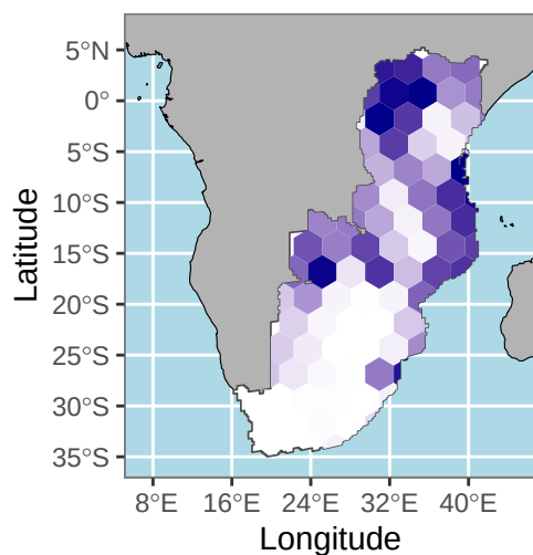
t = 1700 BP
