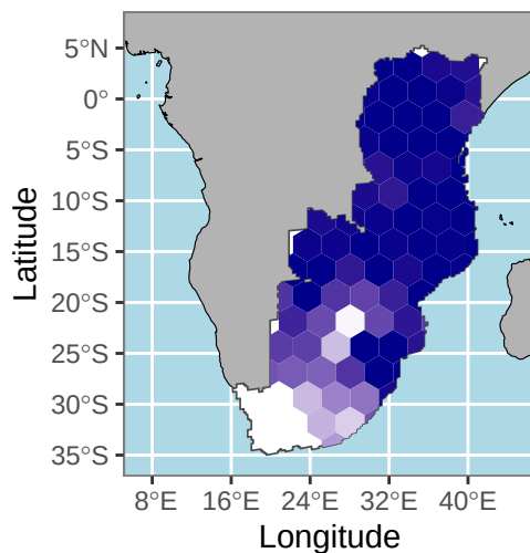
t = 1550 BP
