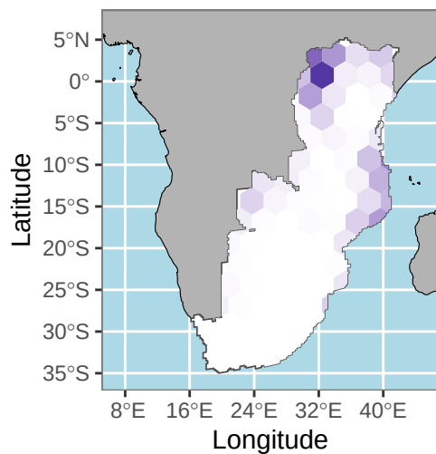
t = 2150 BP
