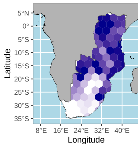
t = 1400 BP
