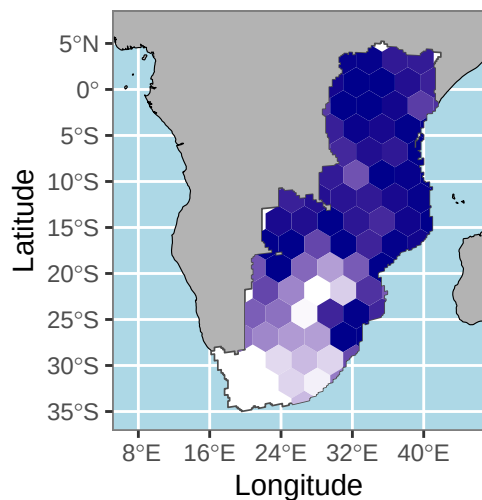
t = 1700 BP
