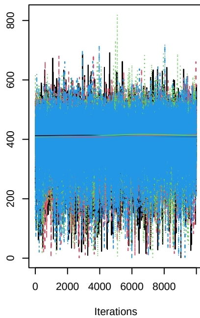
\nabla[24]
