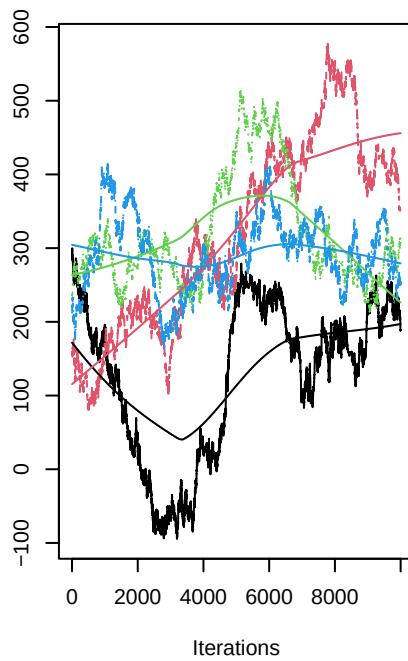
beta2
