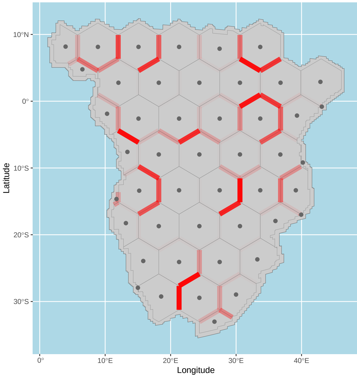
Spatial residue wombling, c = 400 years
