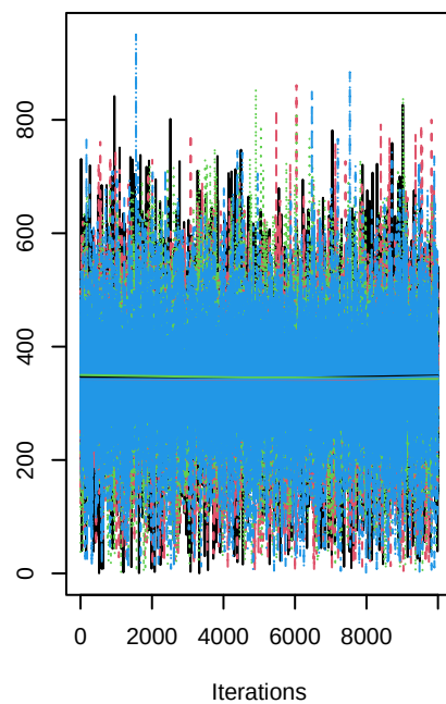
\nabla[24]
