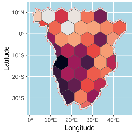
t = 1400 BP
