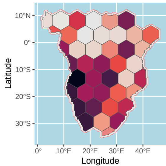
t = 1600 BP
