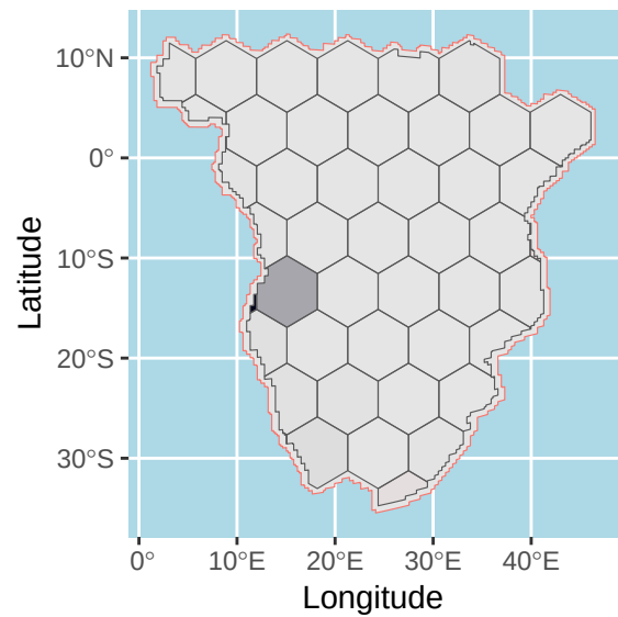
t = 2400 BP
