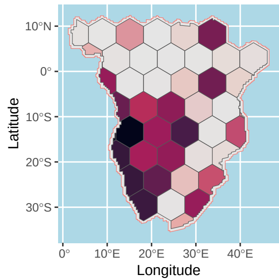
t = 1800 BP
