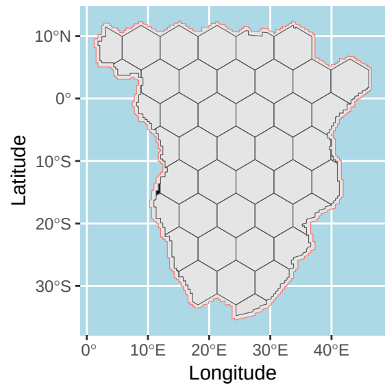
t = 2800 BP
