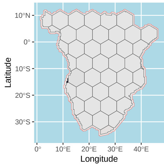
t = 2600 BP
