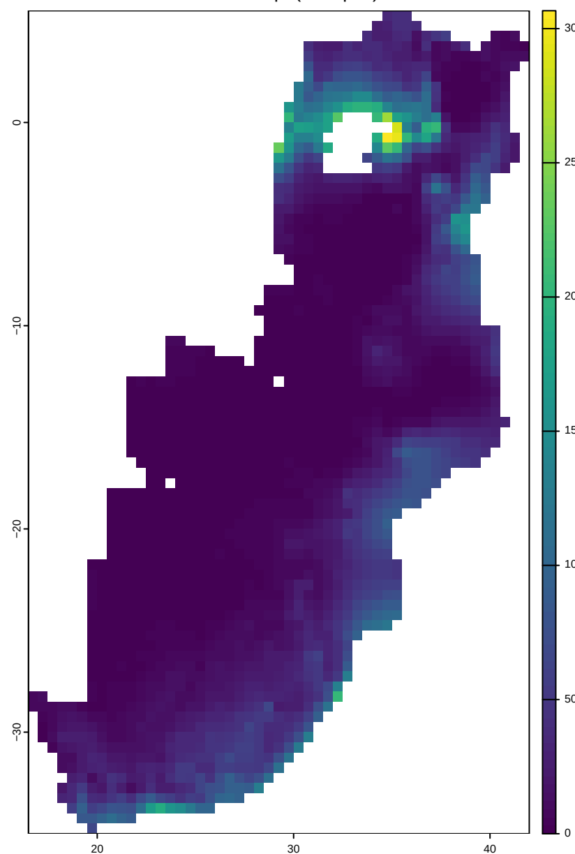
NPP (gC m -2 yr -1 )
