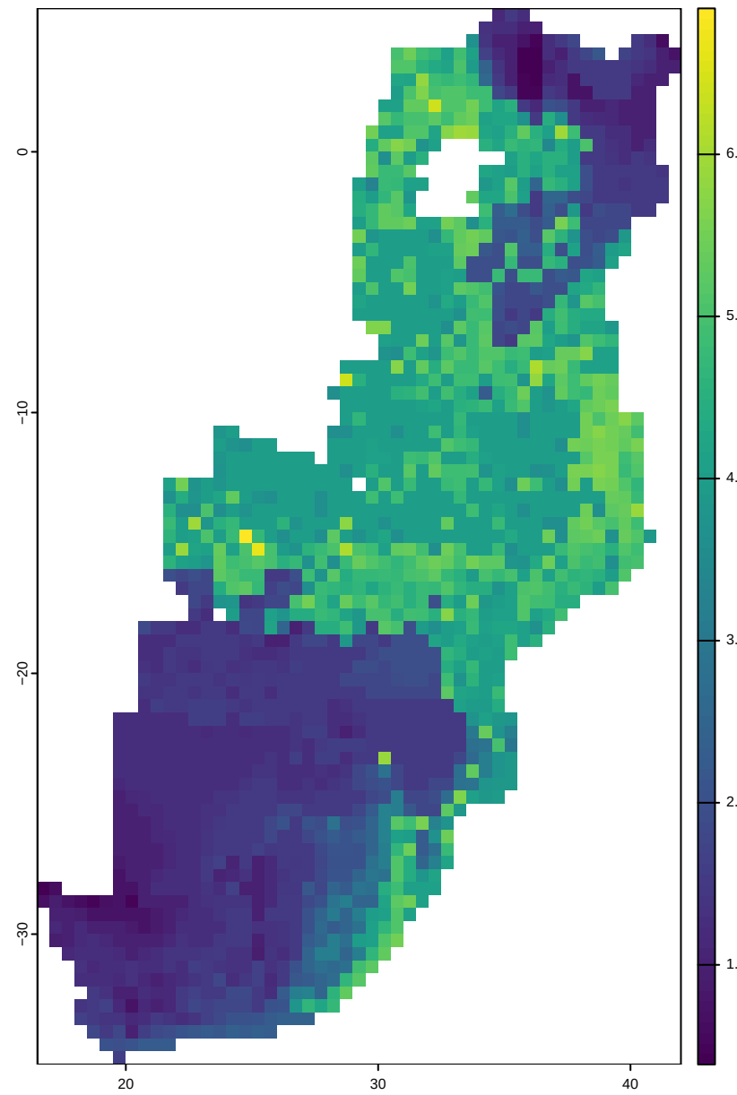
LAI (gC m -2 )
