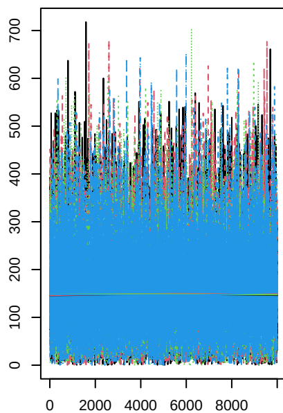
\nabla[24]
