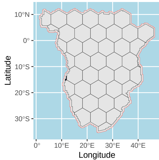
t = 2600 BP
