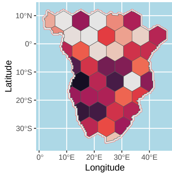
t = 1400 BP
