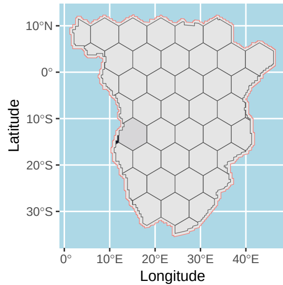
t = 2400 BP
