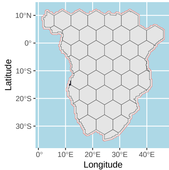
t = 2800 BP
