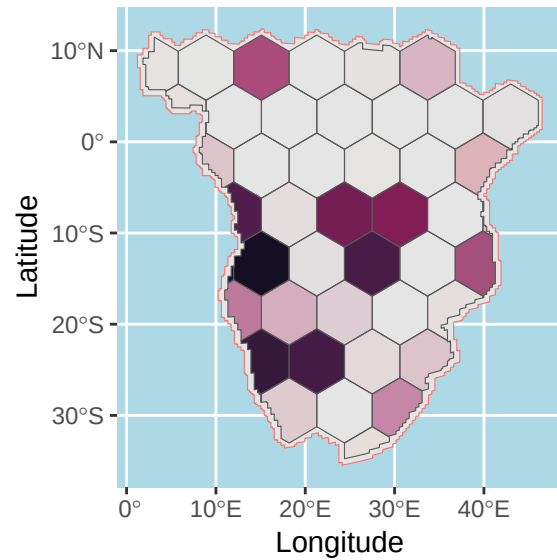
t = 1800 BP
