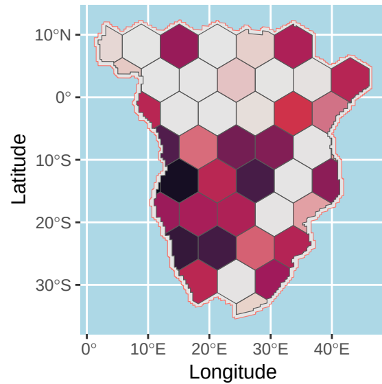
t = 1600 BP
