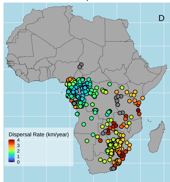
Posterior median of dispersal rate with \tau = 0.99
