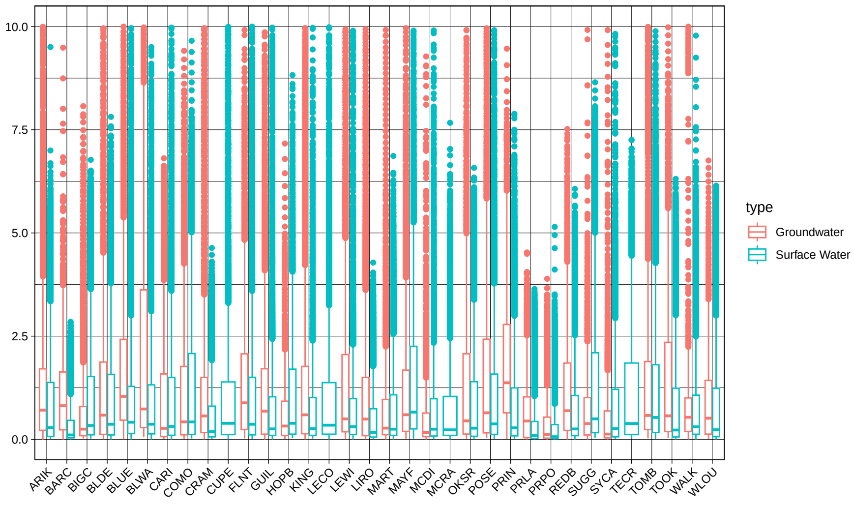
SUVA at 254 nm
