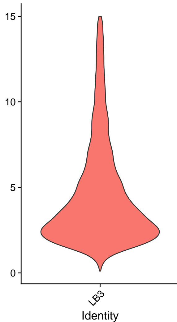
percent.mt
