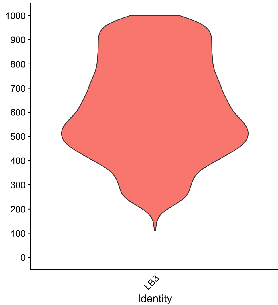
nFeature_RNA
