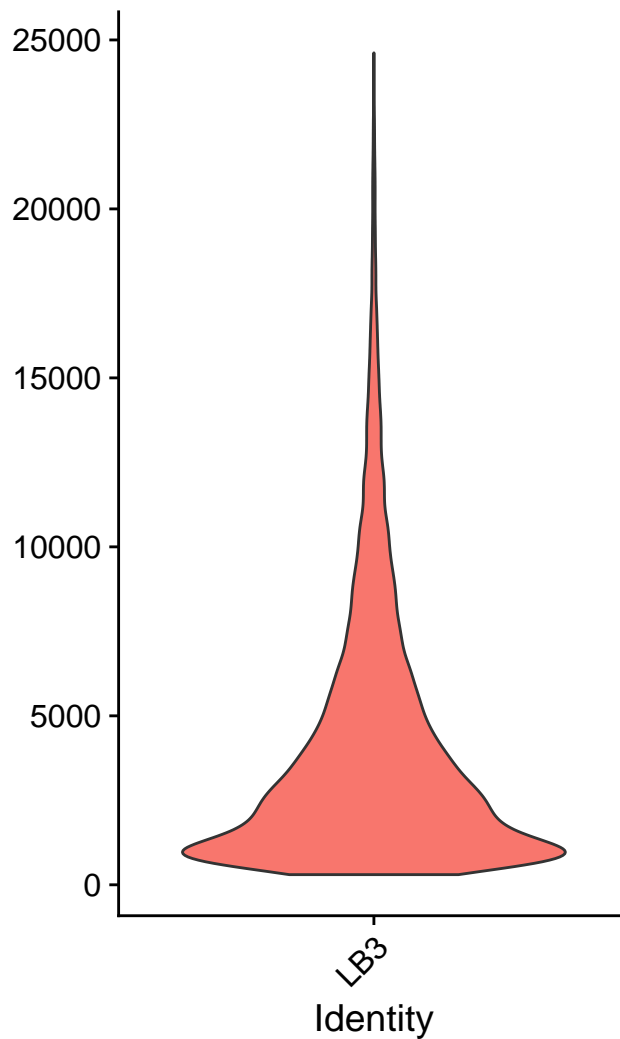
nCount_RNA
