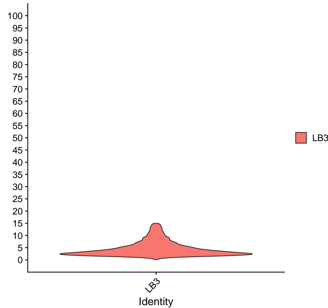
percent.mt
