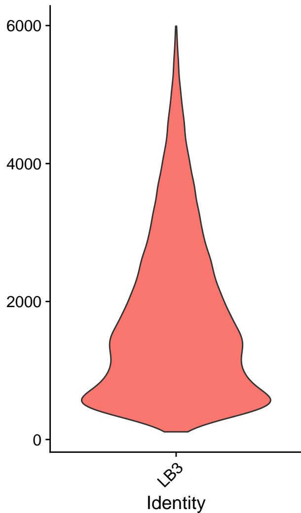
nFeature_RNA
