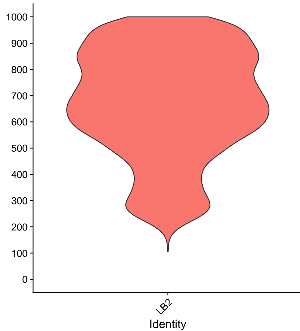
nFeature_RNA
