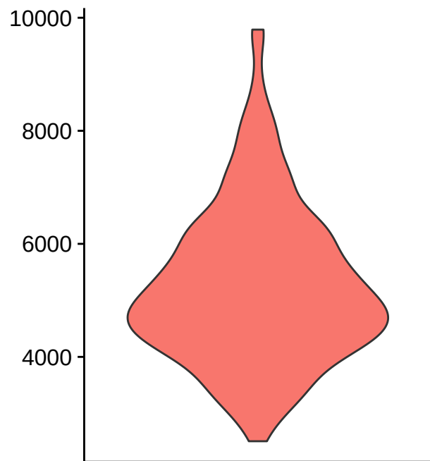
nFeature_RNA
