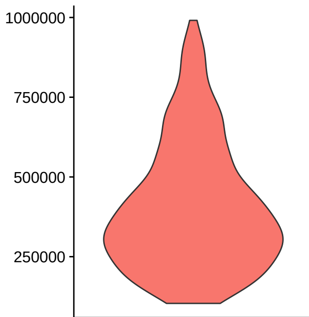
nCount_RNA
