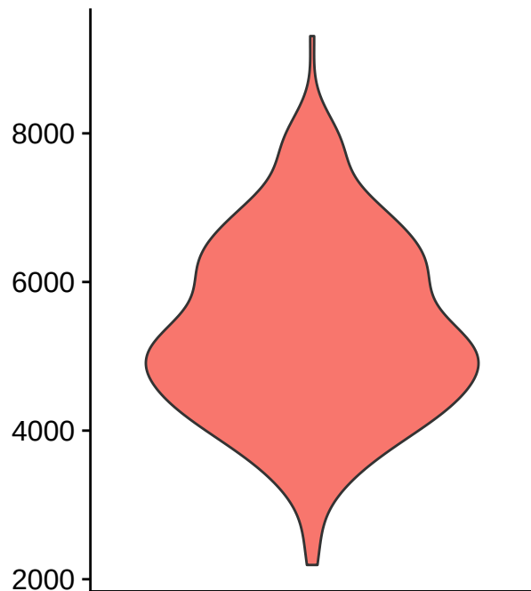
nFeature_RNA
