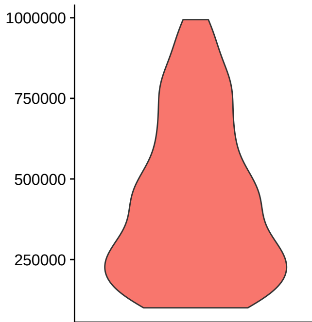
nCount_RNA
