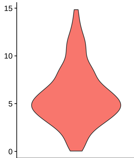
percent.mt
