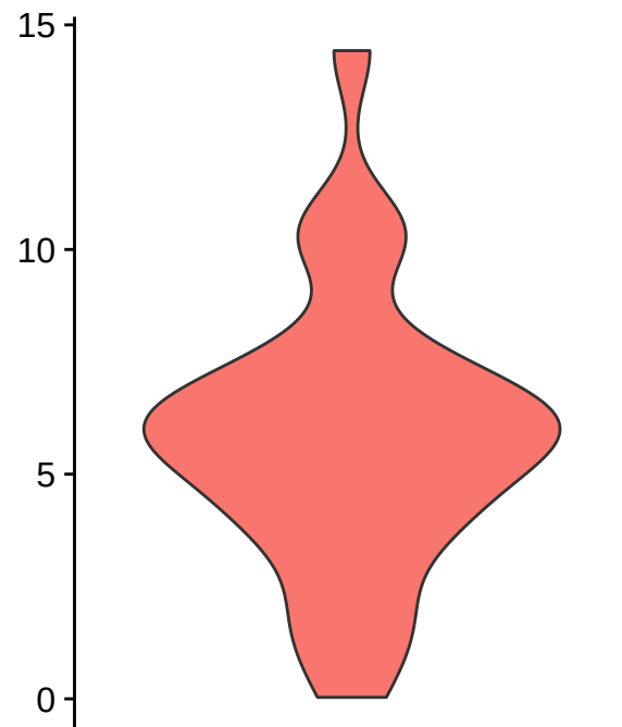
percent.mt
