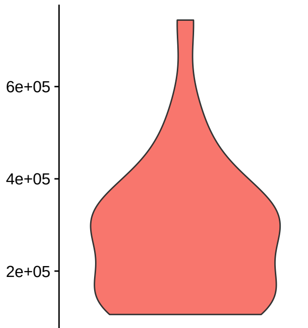
nCount_RNA
