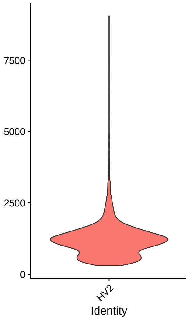
nCount_RNA
