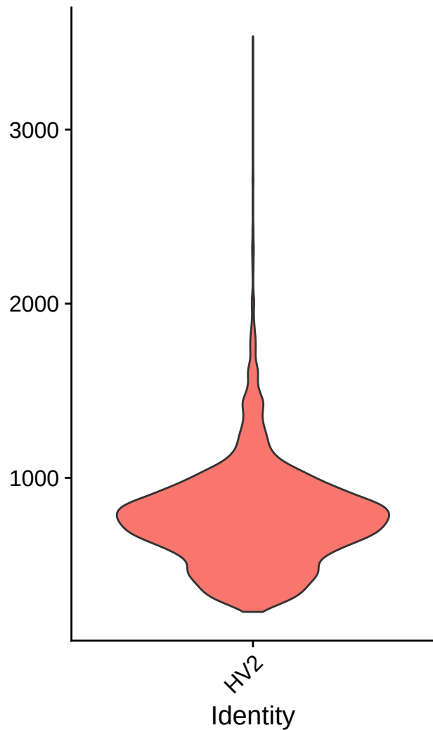
nFeature_RNA
