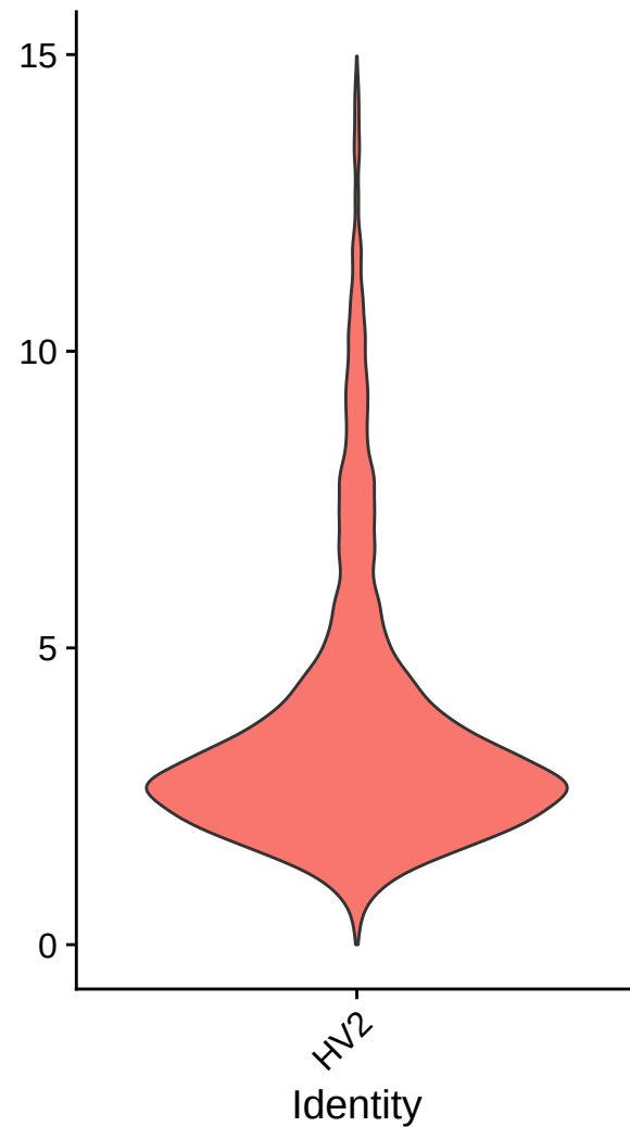
percent.mt
