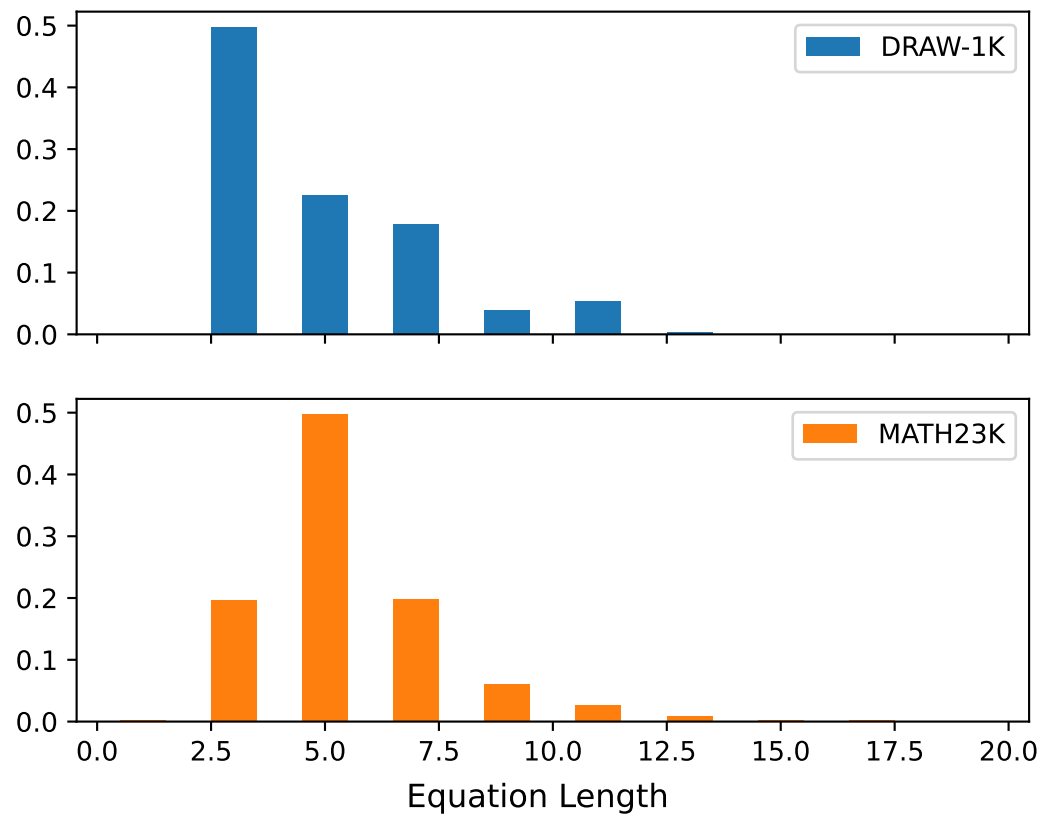
Equation Lengths By Equation Number in DRAW-1K and MATH23K
