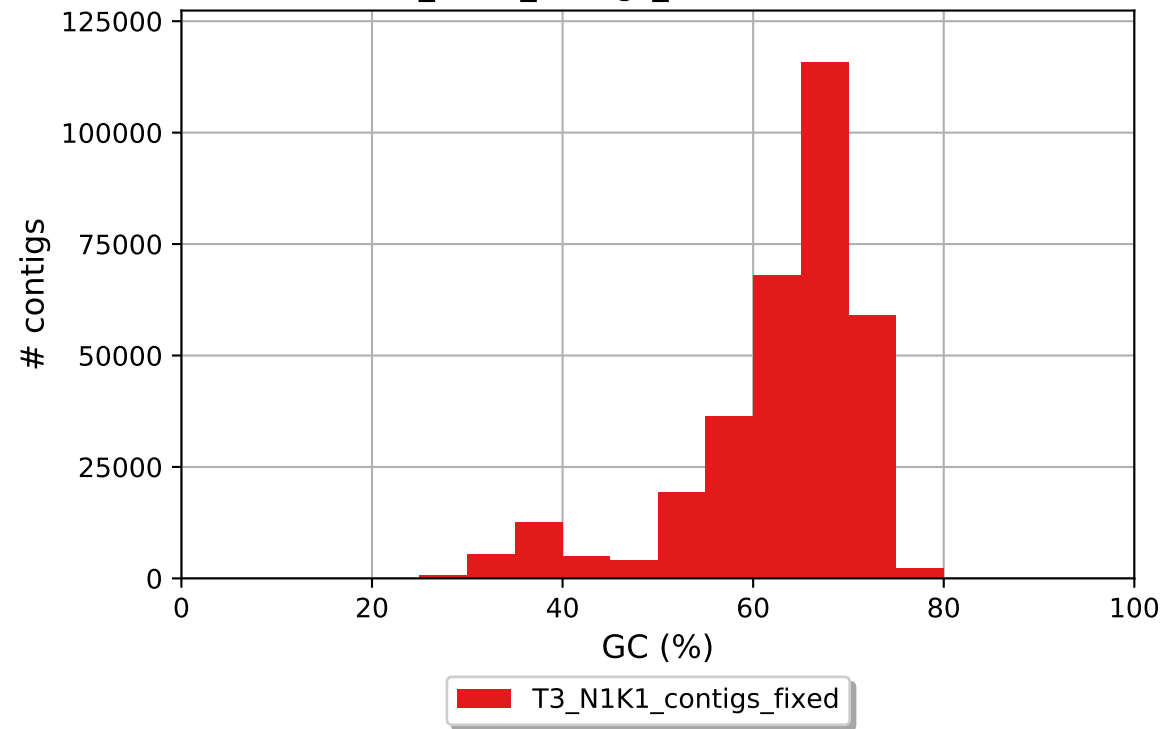
T3_N1K1_contigs_fixed GC content
