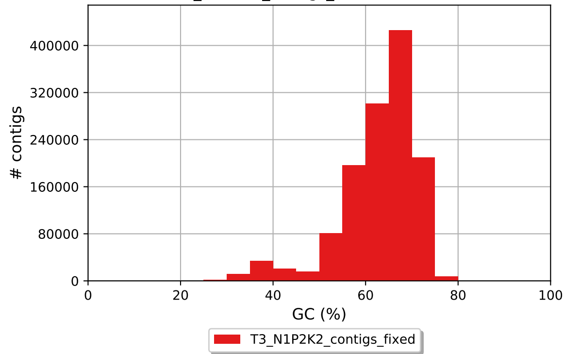
T3_N1P2K2_contigs_fixed GC content
