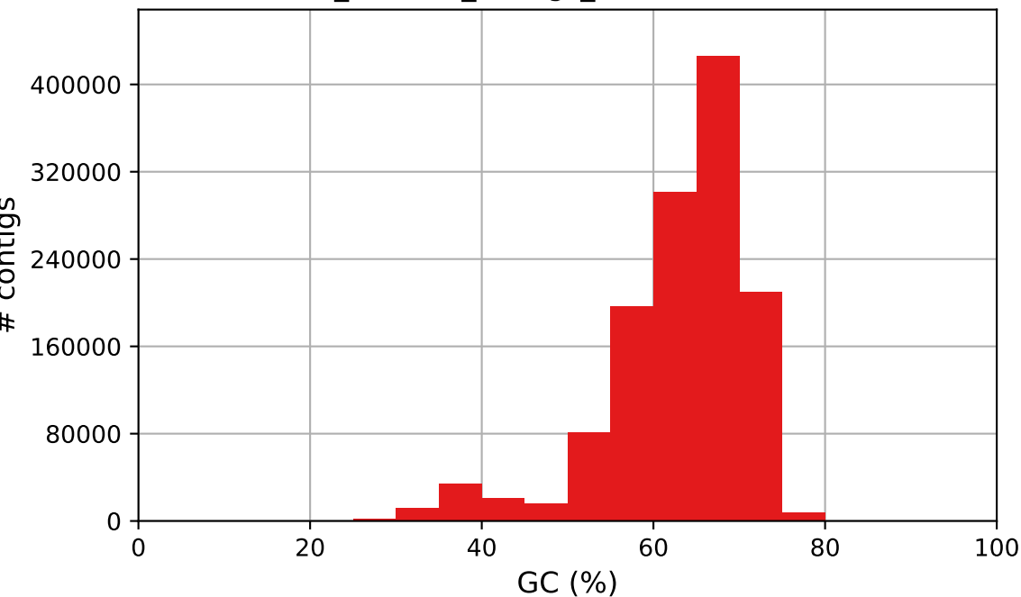
T3_N1P2K2_contigs_fixed GC content
