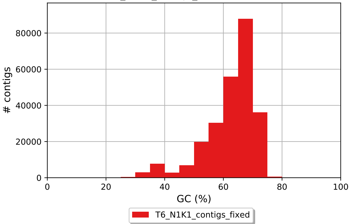
T6_N1K1_contigs_fixed GC content
