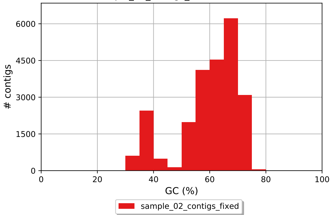
sample_02_contigs_fixed GC content
