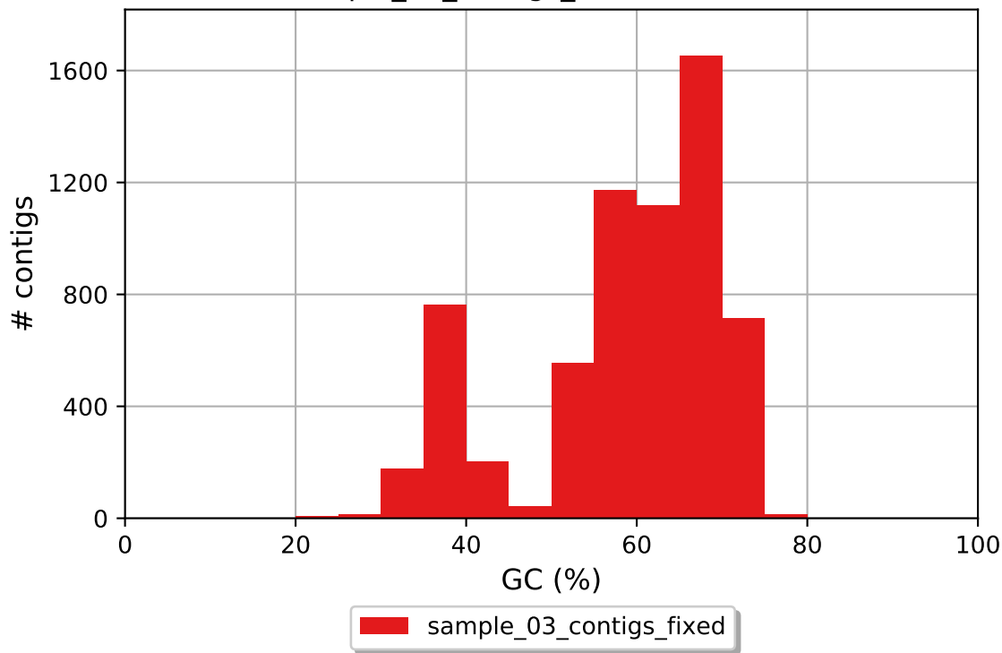
sample_03_contigs_fixed GC content
