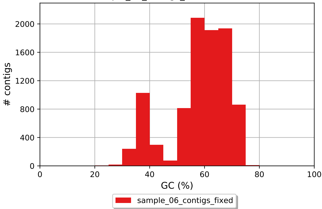
sample_06_contigs_fixed GC content
