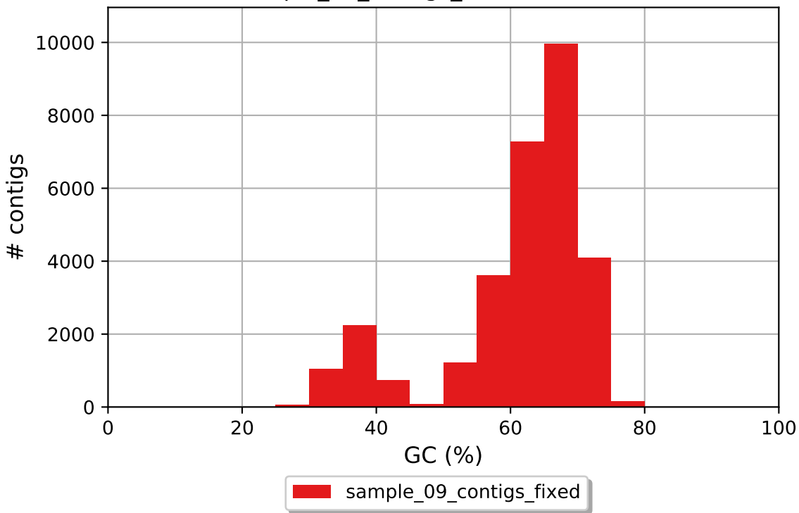
sample_09_contigs_fixed GC content
