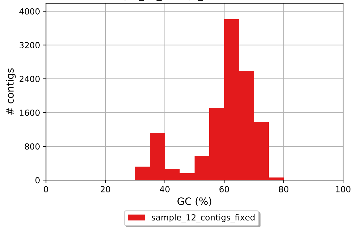
sample_12_contigs_fixed GC content
