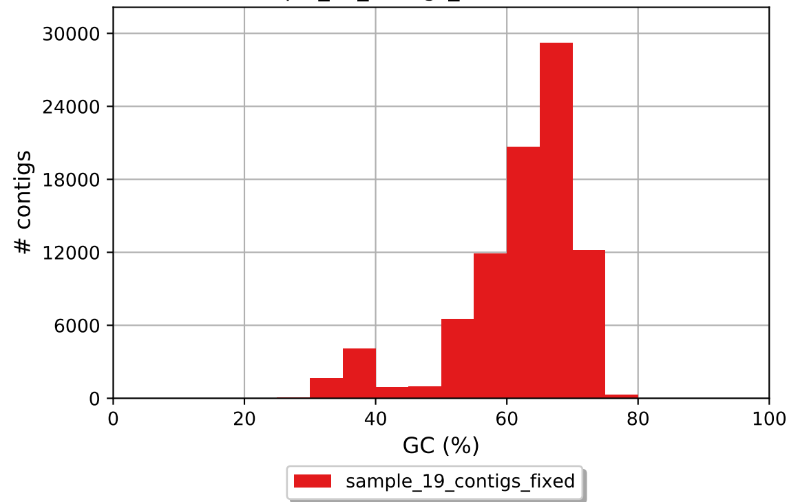
sample_19_contigs_fixed GC content
