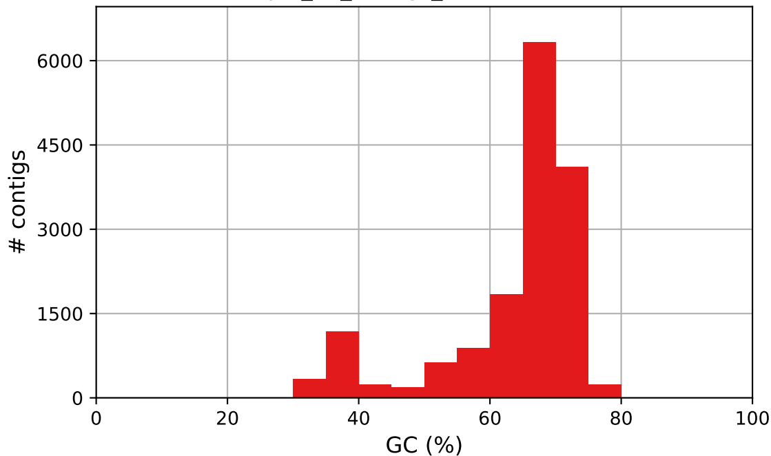
sample_23_contigs_fixed GC content
