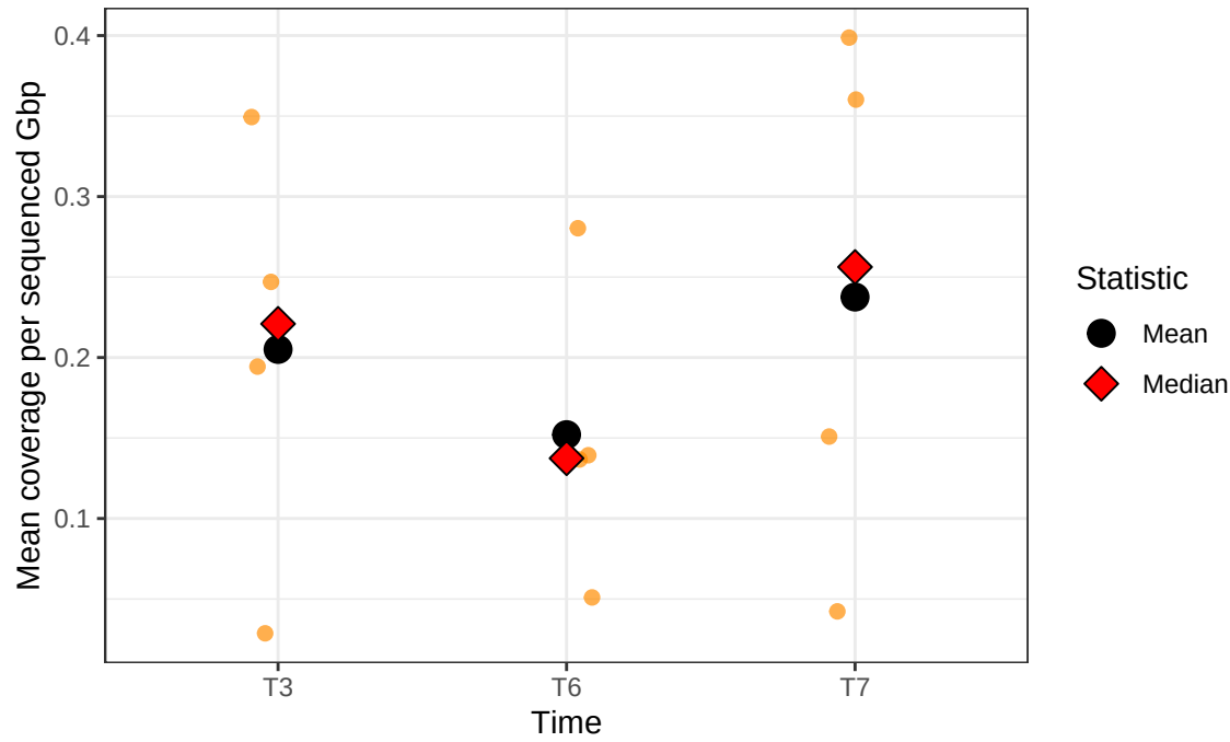
N1K1 – Dotplot
