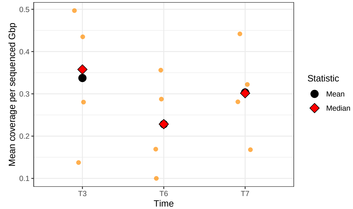
N1P2K2 – Dotplot
