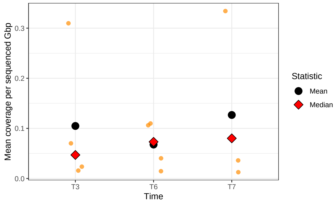
N1K1 – Dotplot
