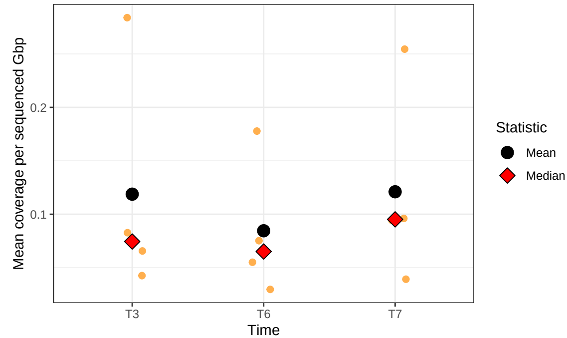
N1P2K2 – Dotplot
