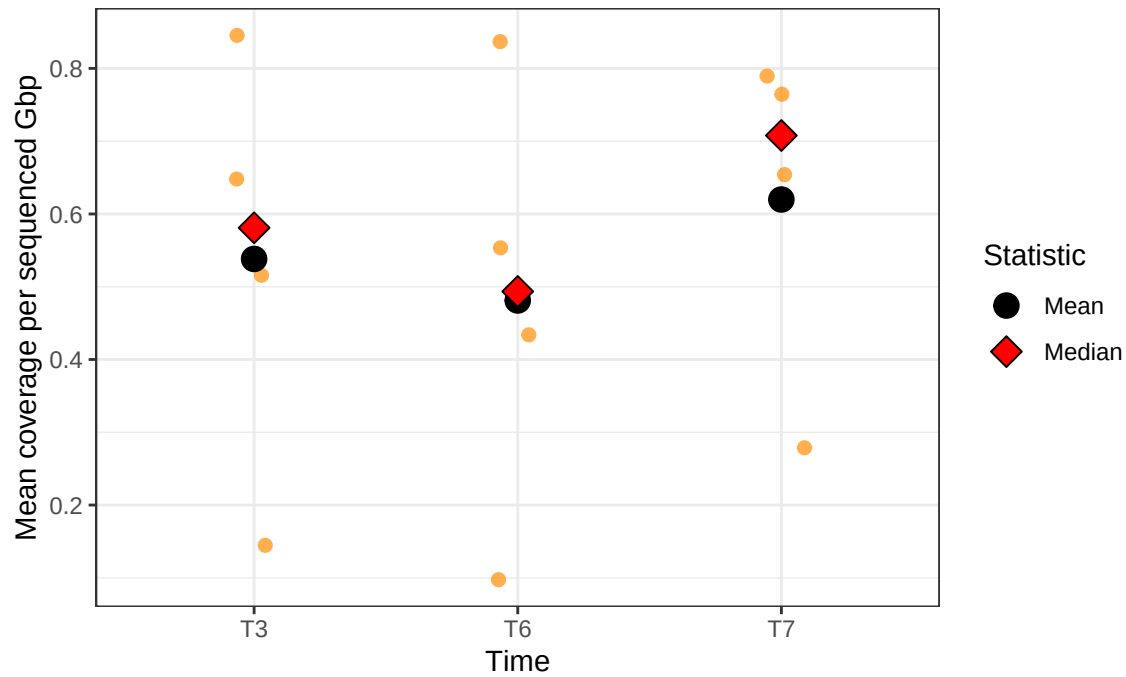
N1P2K2 – Dotplot
