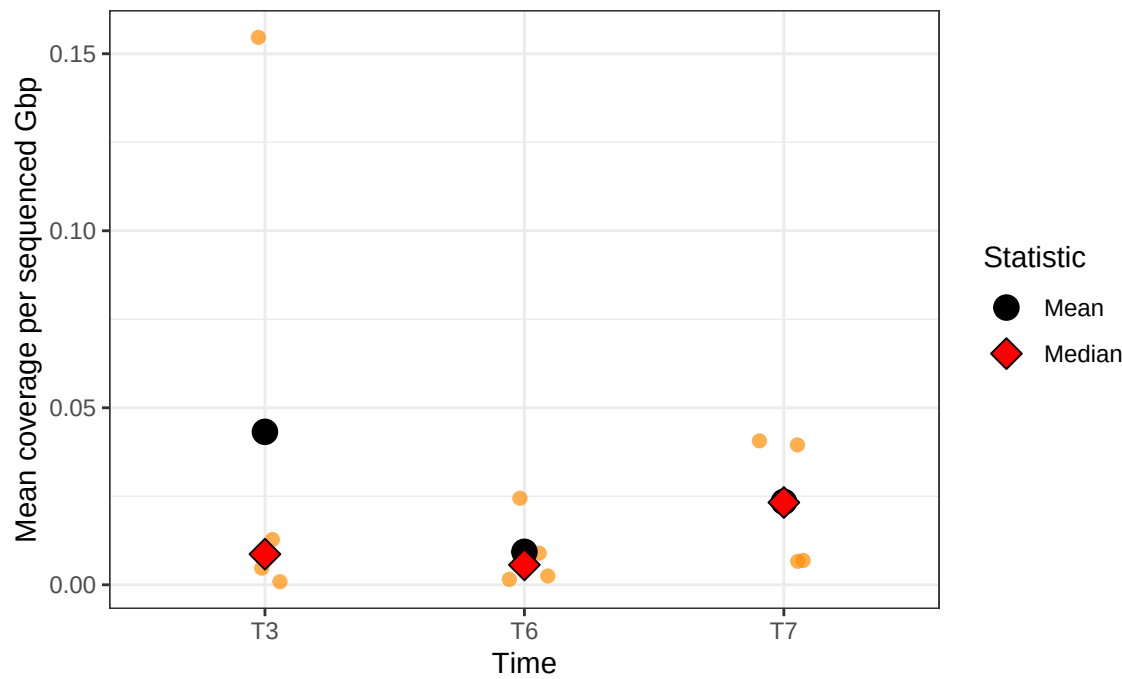
N1P2K2 – Dotplot
