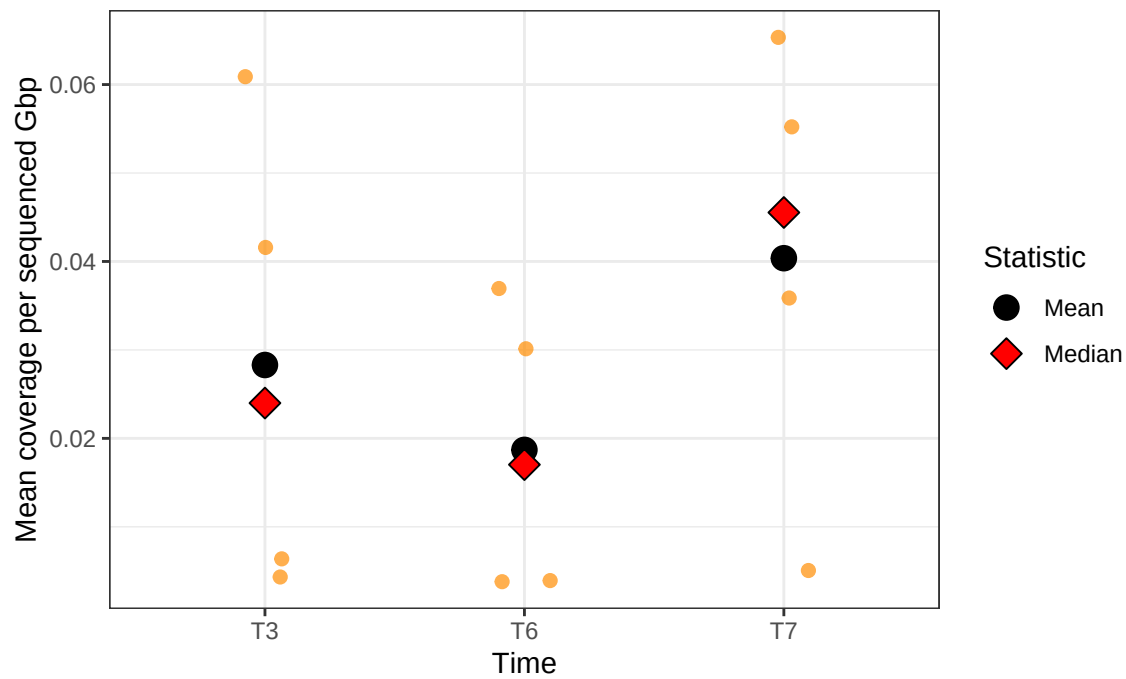
N1P2K2 – Dotplot
