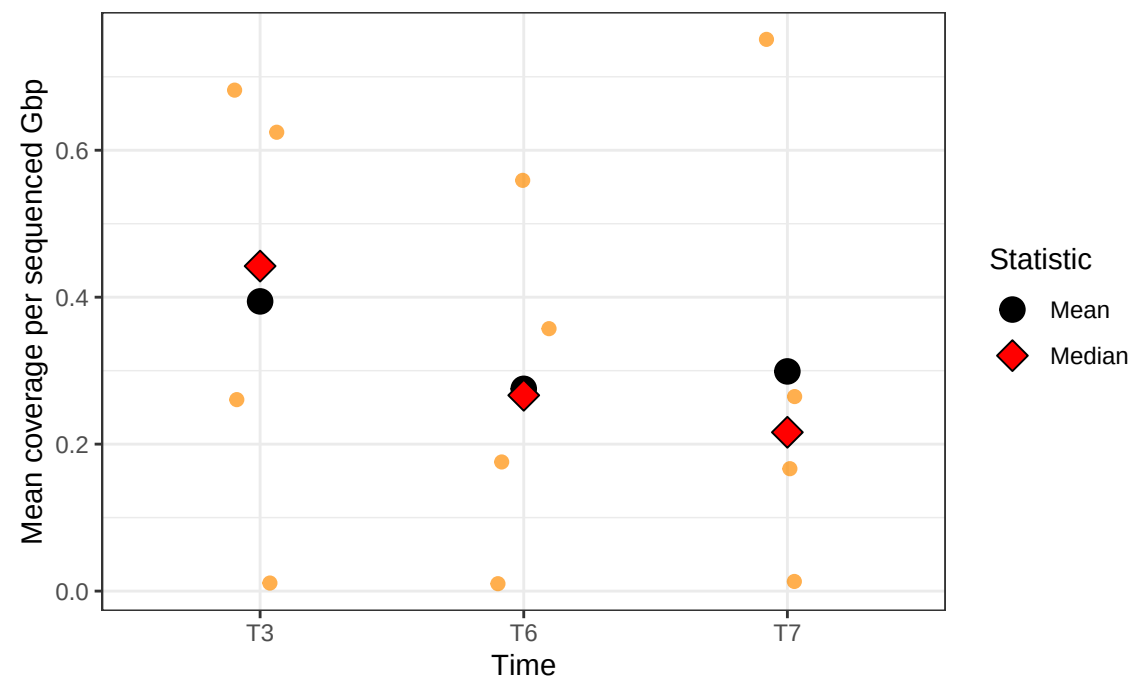
N1P2K2 – Dotplot
