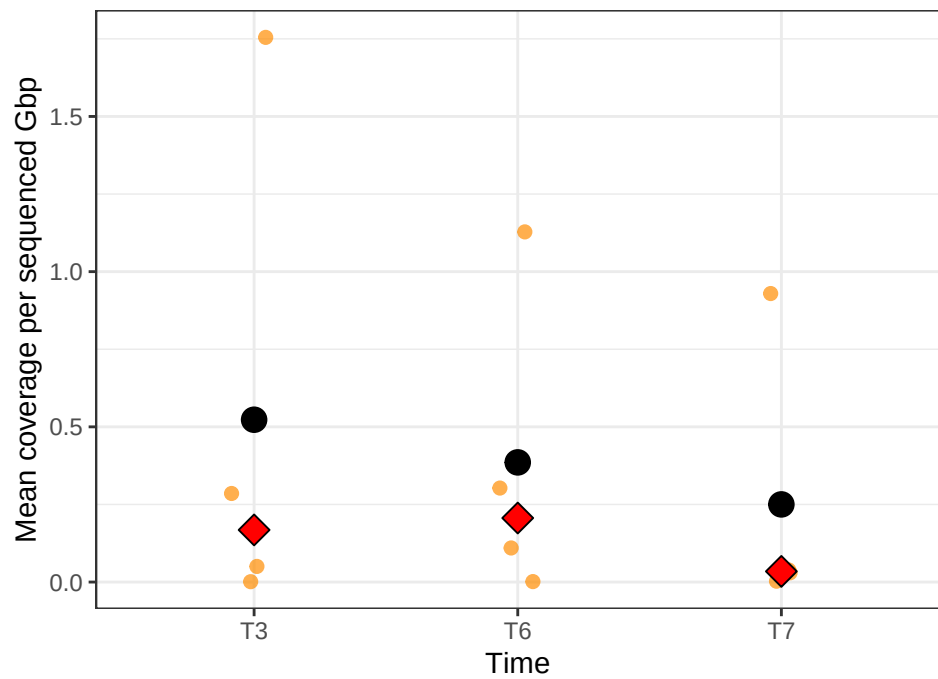
N1K1 – Dotplot
