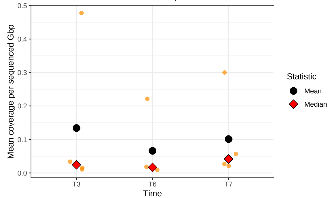
N1P2K2 – Dotplot
