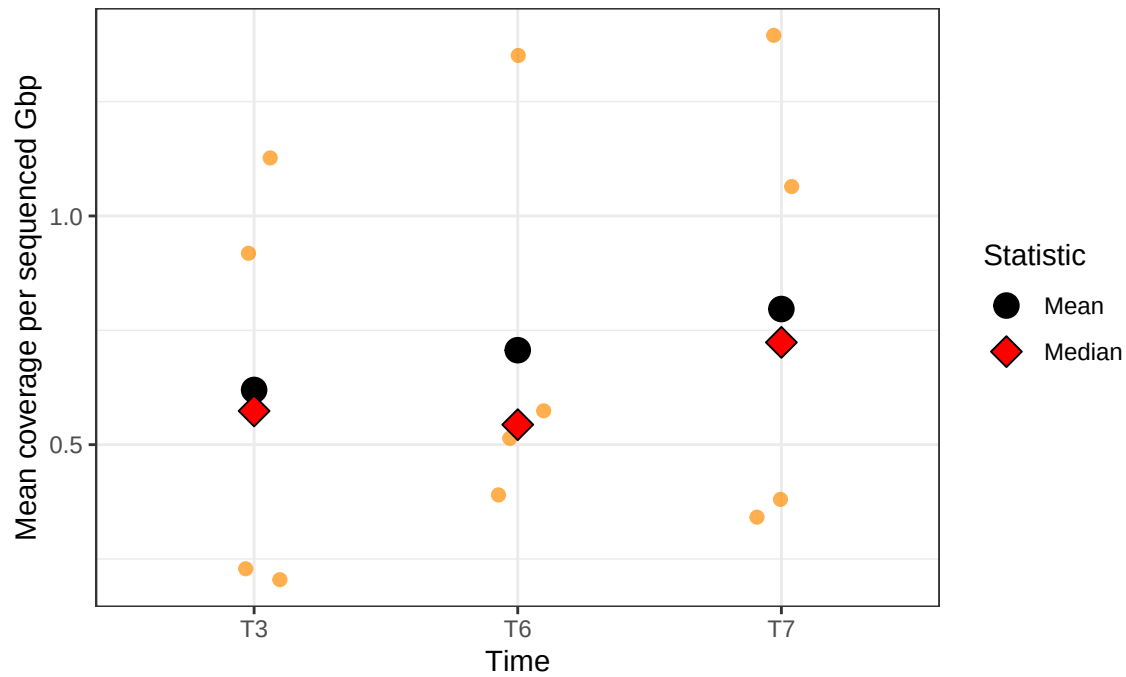
N1K1 – Dotplot
