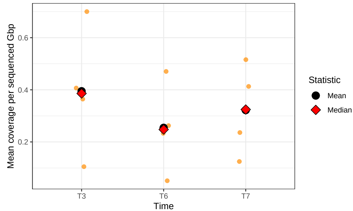
N1P2K2 – Dotplot
