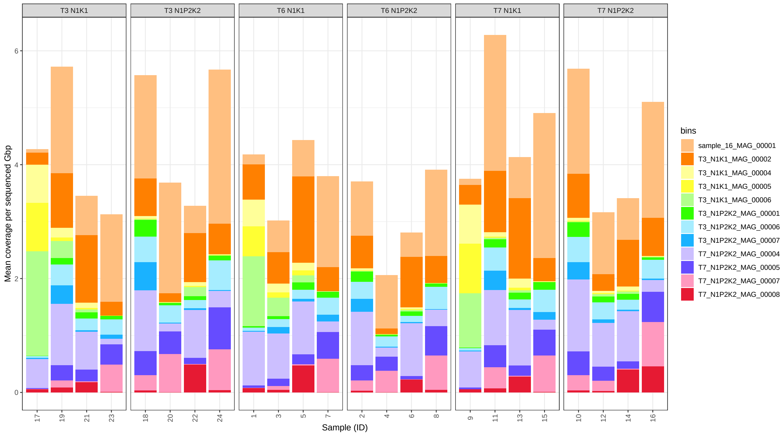
Mean coverage per sequenced Gbp (stacked by MAGs)
