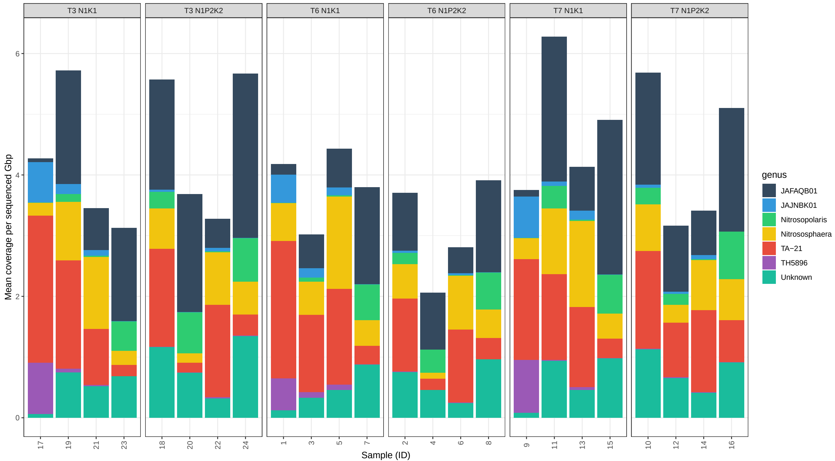
Mean coverage per sequenced Gbp (stacked by genus)
