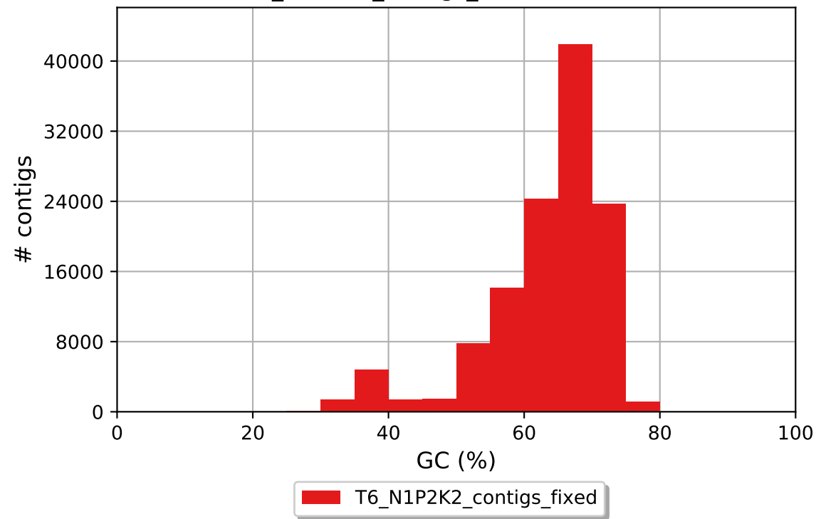
T6_N1P2K2_contigs_fixed GC content
