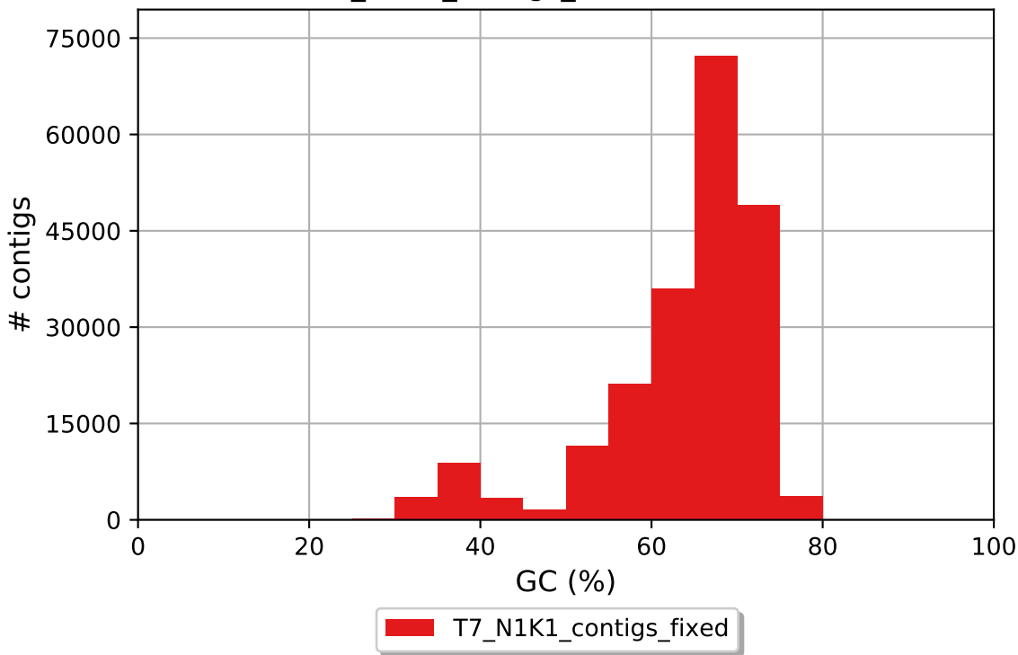
T7_N1K1_contigs_fixed GC content
