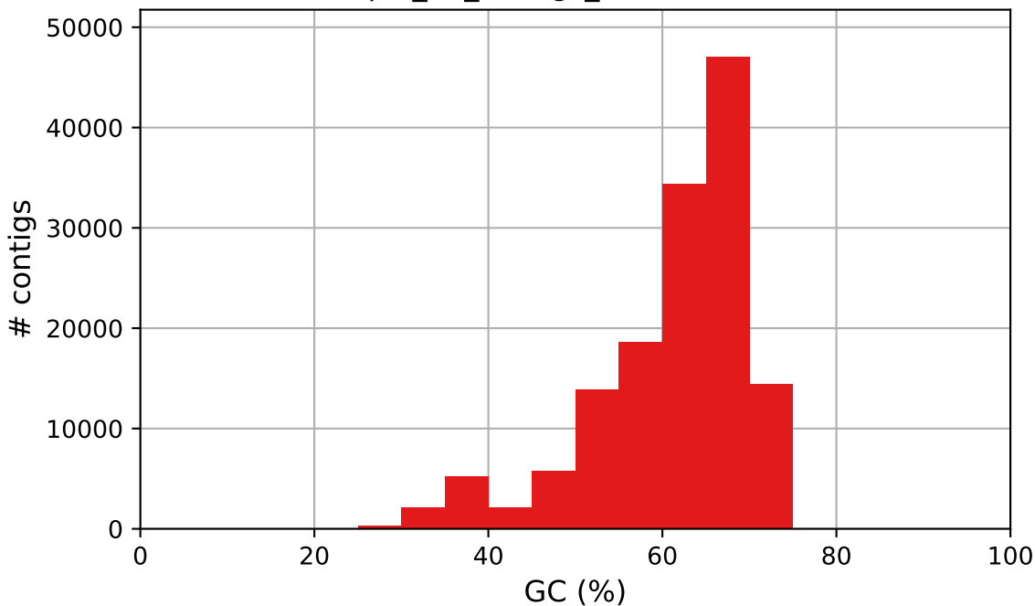
sample_01_contigs_fixed GC content
