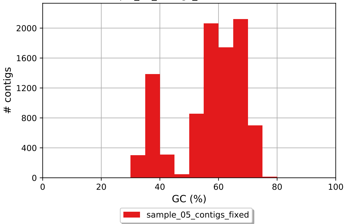
sample_05_contigs_fixed GC content
